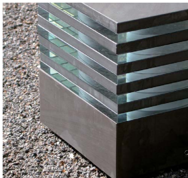
Type greywacke
